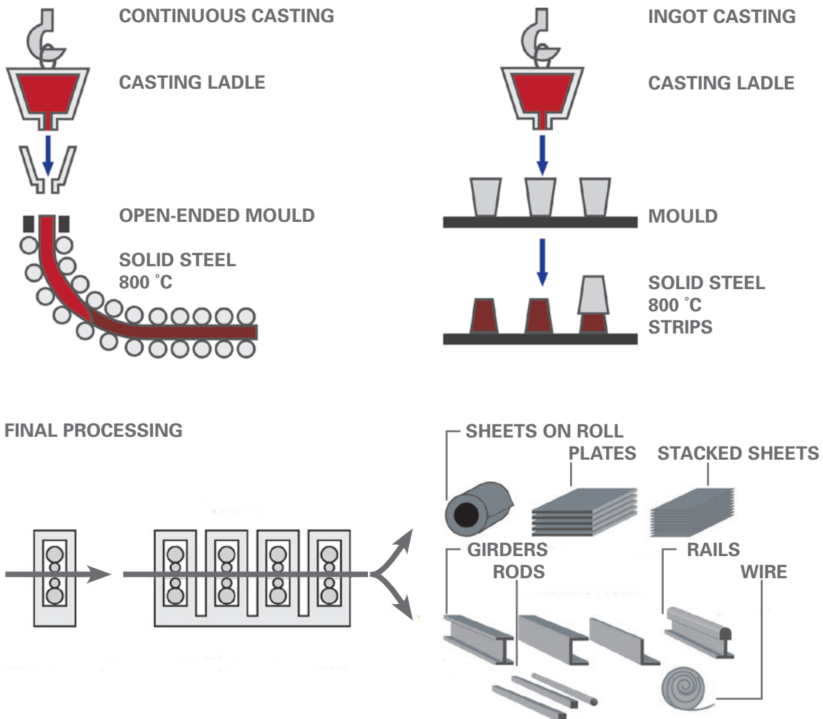
Graphic 7: Comparison continuous casting to ingot casting
