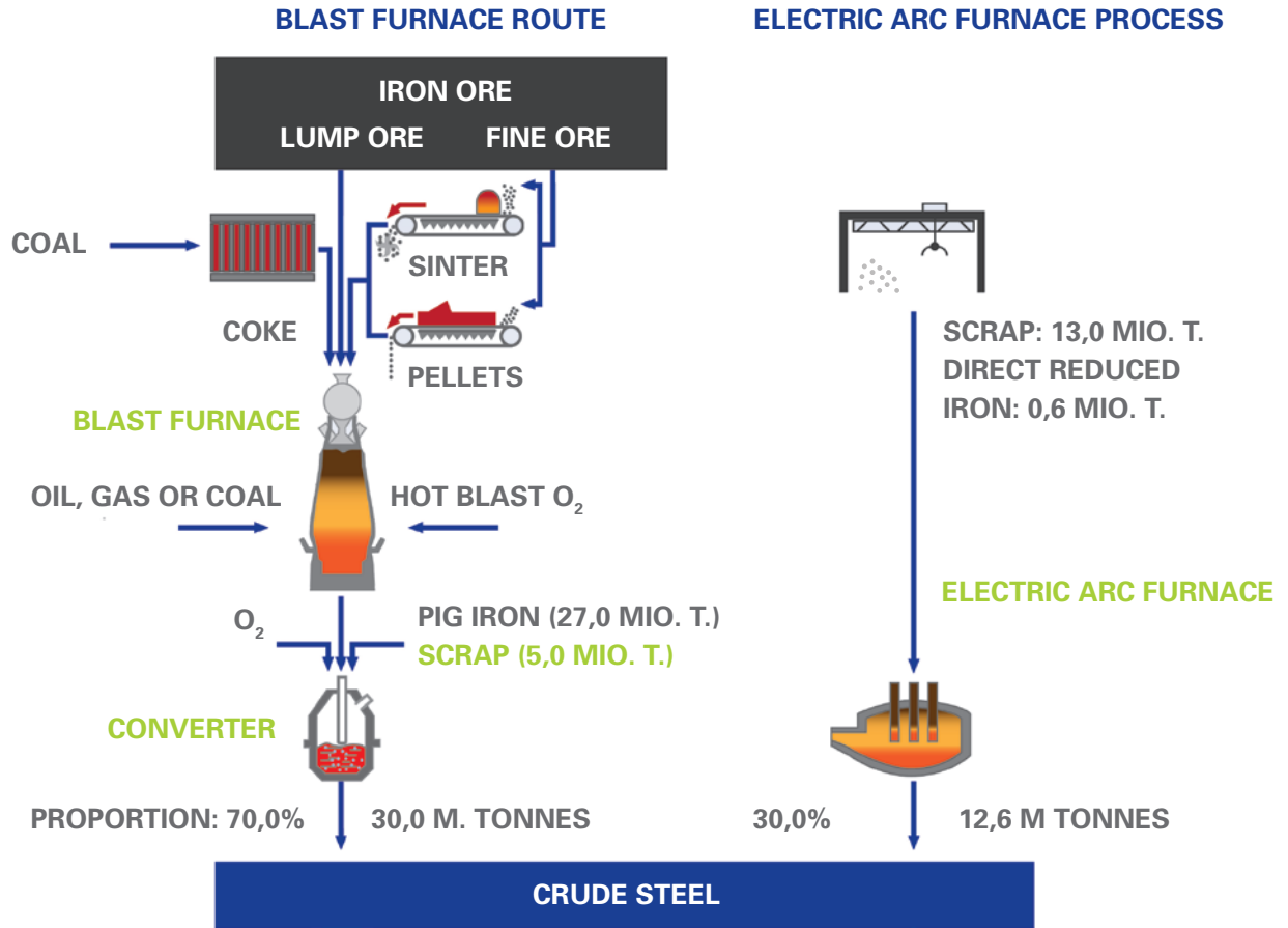
Graphic 6: Facts on steel production during 2017
