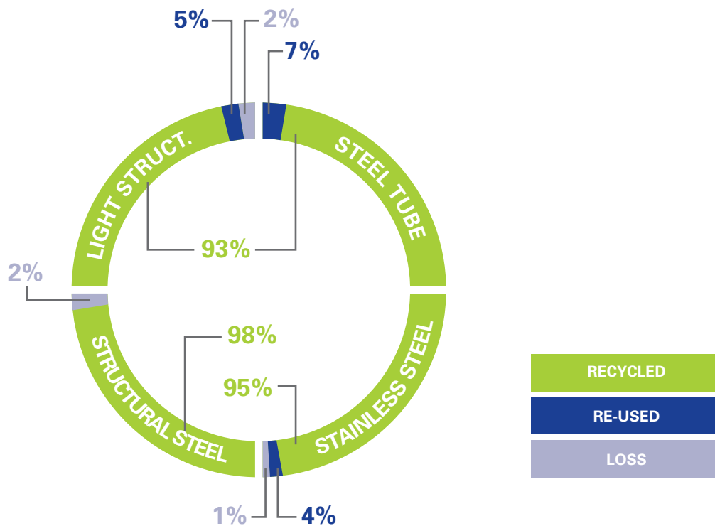
Graphic 5: Summary of the re-use and recycling rates of steel Eurofer-Study of 2012 (excerpt)
