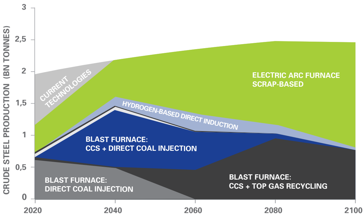
Graphic 18: Technology competition in the binding climate target scenario (3.5 F scenario) for Demand Stagnation in 2050
